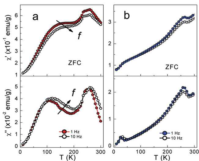
Figure 4. Temperature dependence of \chi' and \chi'' for the FMO NCs/SiO 2 /Si sample (a) and for oleic acid-coated FMO NCs for the drop casting (b) in the ac field h = 3.8 Oe and at both the frequency f = 1 and 10 Hz.
