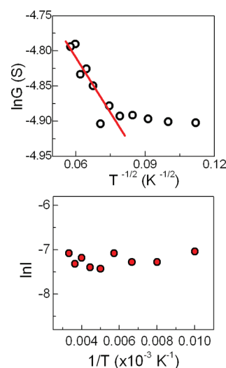
Figure 6. Temperature dependence of G at 0.4 V (upper panel) and \ln I versus 1/T plot (lower panel).
