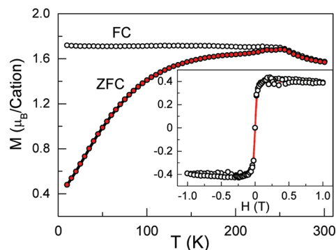
Figure 3. Field dependence at 300 K (the inset) and temperature dependence in H = 100 Oe of magnetization of the FMO NCs/SiO 2 /Si sample.
