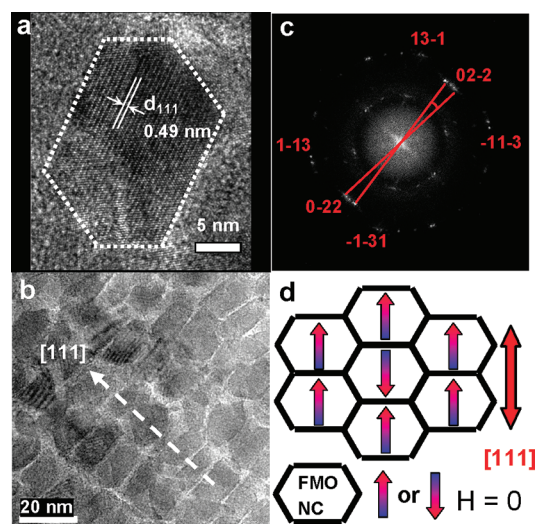
Figure 1. (a) TEM image of an FMO NC coated with oleic acid. Dotted line surrounding the NC is a guide for eye. (b) Cross-sectional TEM image of the FMO NCs/SiO 2 /Si sample. (c) FFT pattern for all the area of the image b. Indices of distinctive FFT spots with the incident beam direction along the [-2\ 1\ 1] axis are overlapped, and crystallographic orientation distribution ( \sim 10^\circ ) is represented by crossed bars. (d) Schematic representation of hexagonally ordered collinear ferromagnetic moments. The ferromagnetic moment of single domain FMO NCs align parallel to the \langle 111 \rangle direction.
