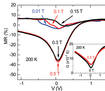
Figure 7. G versus V plot in H = 0 and 0.5 T (the inset) and MR in H = 0.01, 0.1, 0.15, 0.3, and 0.5 T at 200 K.
