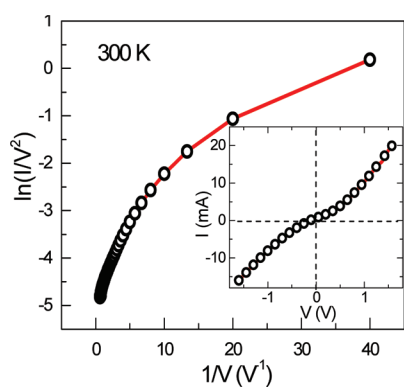
Figure 5. I – V characteristics measured at 300 K in H = 0 (the inset) and Fowler–Nordheim plot of the I – V curve.
